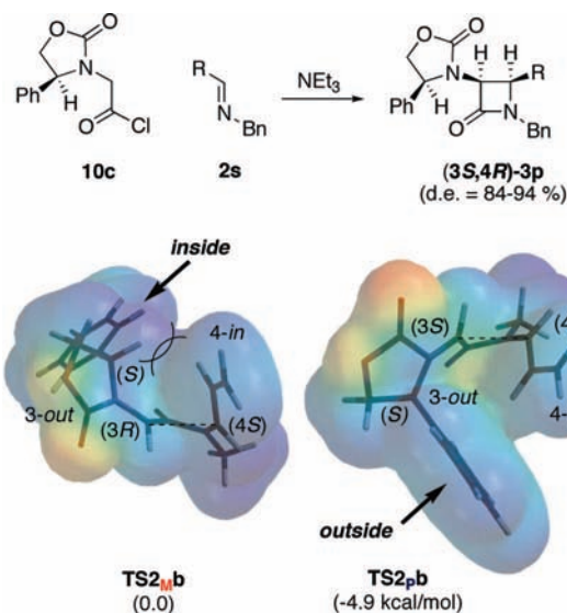
FIGURE 7. A selected example of high diastereoselection induced from the C3 position of the \beta -lactam to be formed: RHF/AM1 geometries and relative enthalpies for saddle points TS2_{Mb} and TS2_{Pb} .
